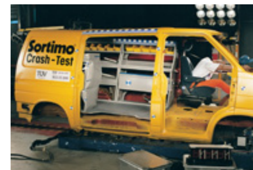
2000: sled test with Sortimo in-vehicle equipment at TÜV Munich
